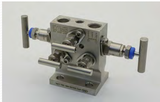
5-WAY MANIFOLD (Single Flange)
